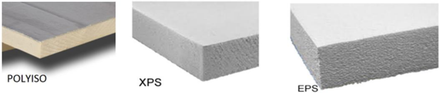
FIGURE 1. EXAMPLES OF POLYISO, XPS, AND EPS FPIS
